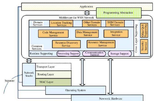
Fig 2- Reference Model of WSN Middleware
